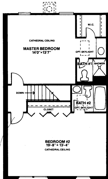
ALTERNATE SECOND FLOOR PLAN
