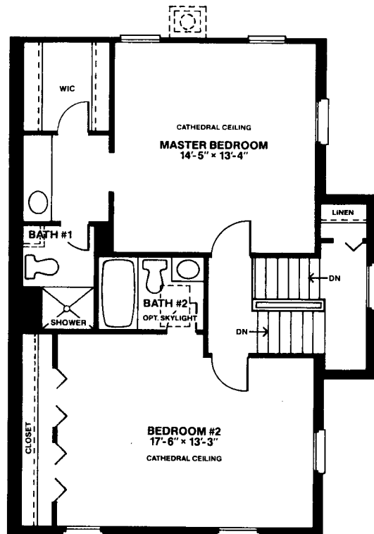
ALTERNATE SECOND FLOOR PLAN
