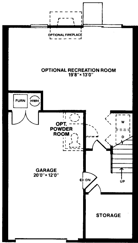
BASEMENT PLAN
