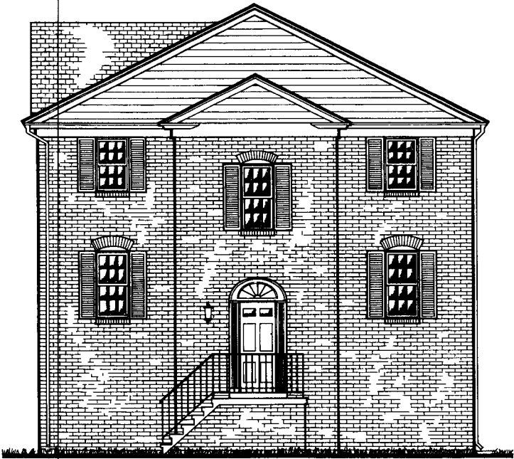
O-1 END UNIT WITH BRICK SIDE OPTION
