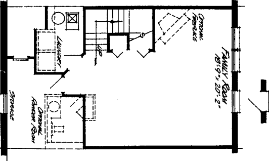
Basement Plan w/Family Room
